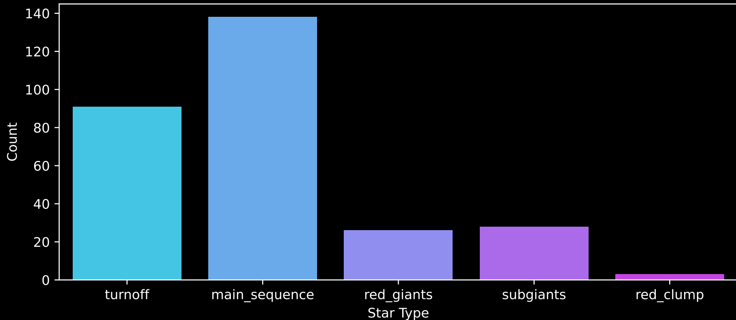
GALAH DR4 Field: [827] Count plot of Star Type
