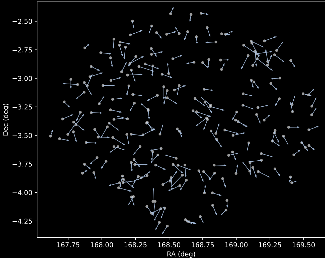
GALAH DR4 Cluster 1 Proper Motion Vectors (n=216)
