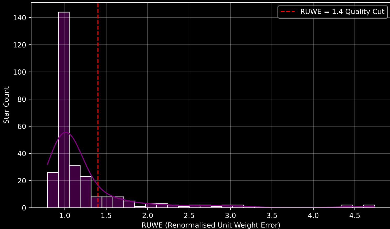
GALAH DR4 Field [827] RUWE Distribution (n= 277)
