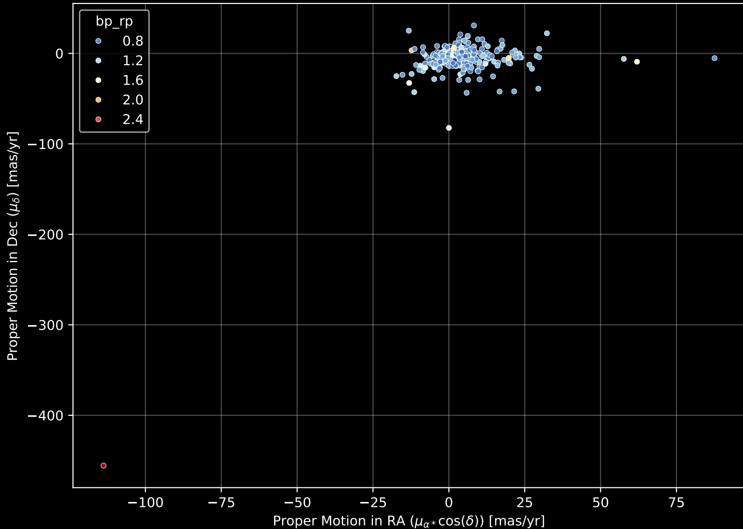
GALAH DR4 Field: [827] Proper Motion Diagram (n= 286)
